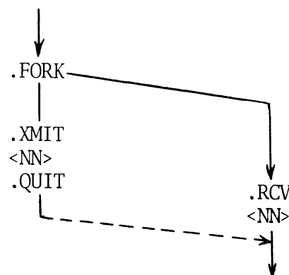
Figure 1-4 Inter-TASK Communication
