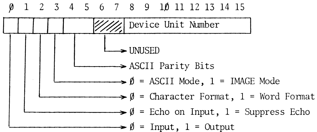
Figure 1-3 Teletype Device Control Word Format
