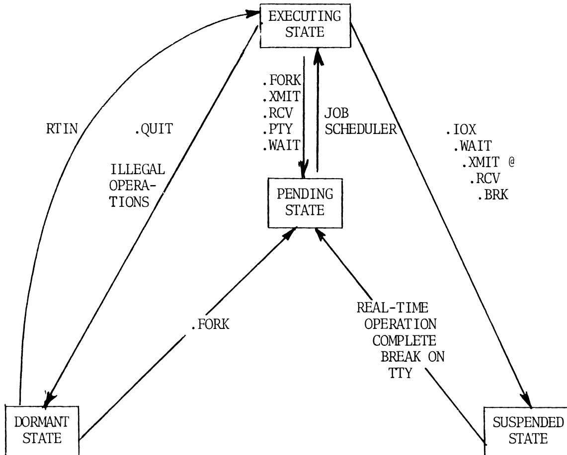
Figure 1-2 TASK STATE TRANSITION
