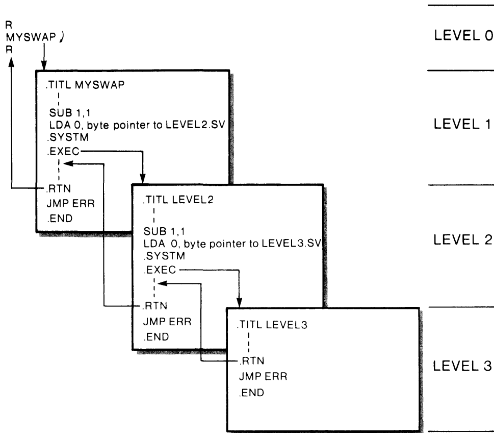
Figure 4.1 Program swapping
