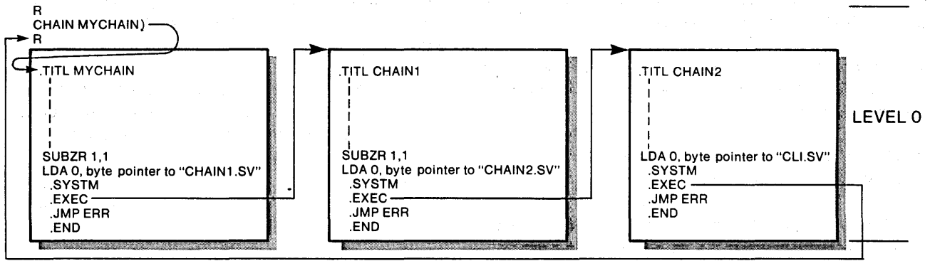
Figure 4.2 Program chaining
