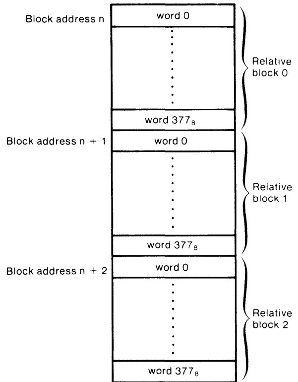
Figure 2.3 Contiguous file block organization SD-00536
