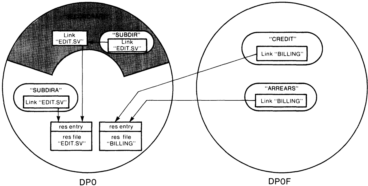
Figure 2.5 Link entries
