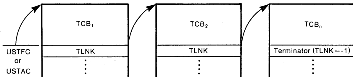
Figure 5.2 TCB chain
