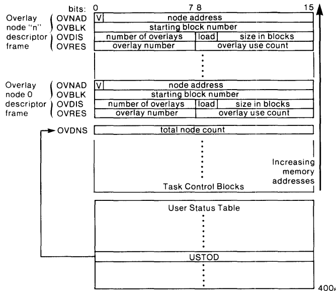
Figure D.1 Overlay directory structure (multitask) SD-00532
