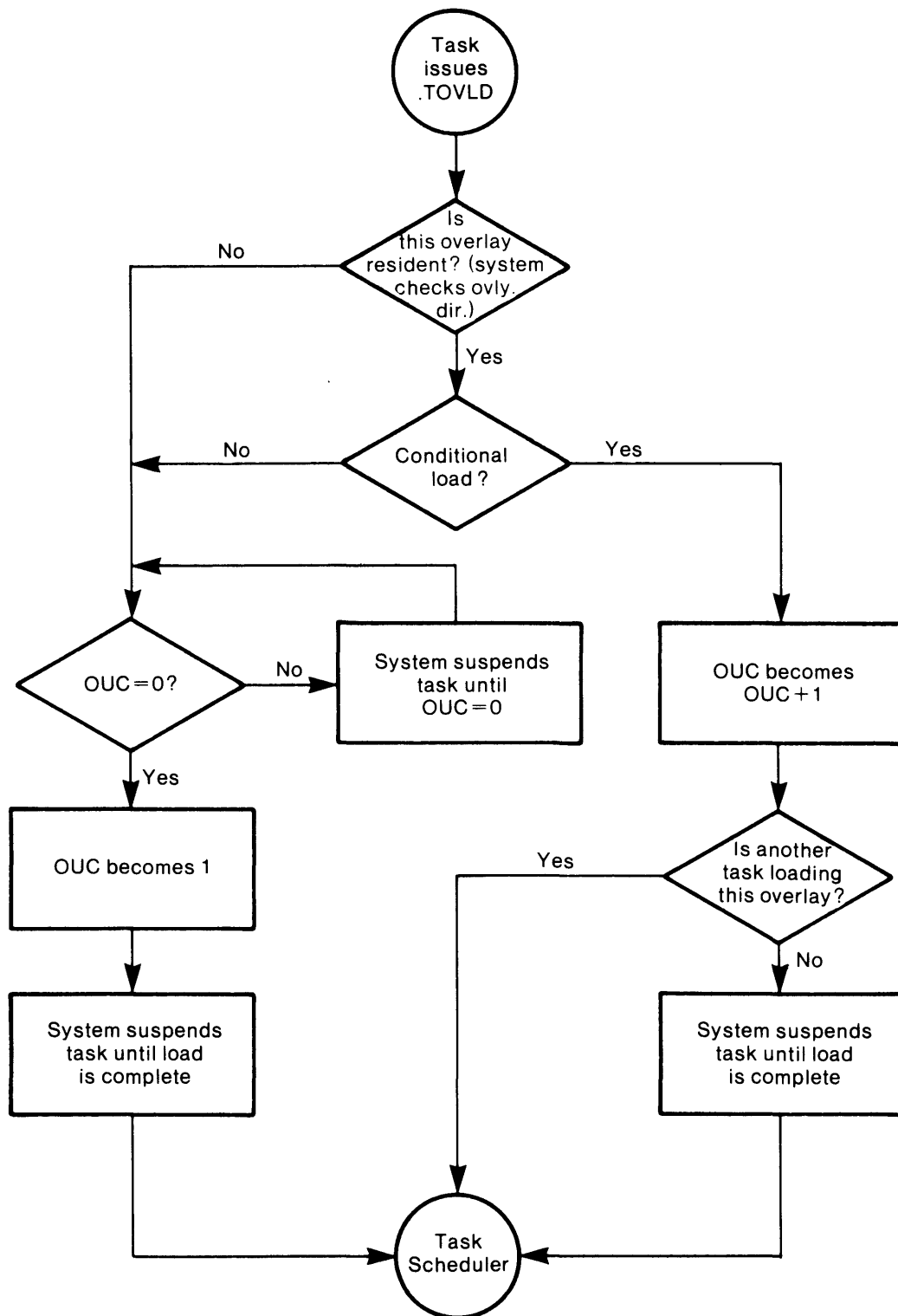
Figure 5.3 TOVLD logic sequence
