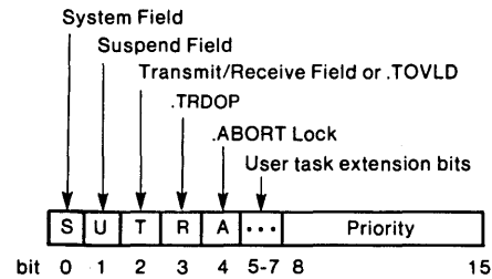
Figure 5.1 Task state/priority information (TPRST) SD-00541
