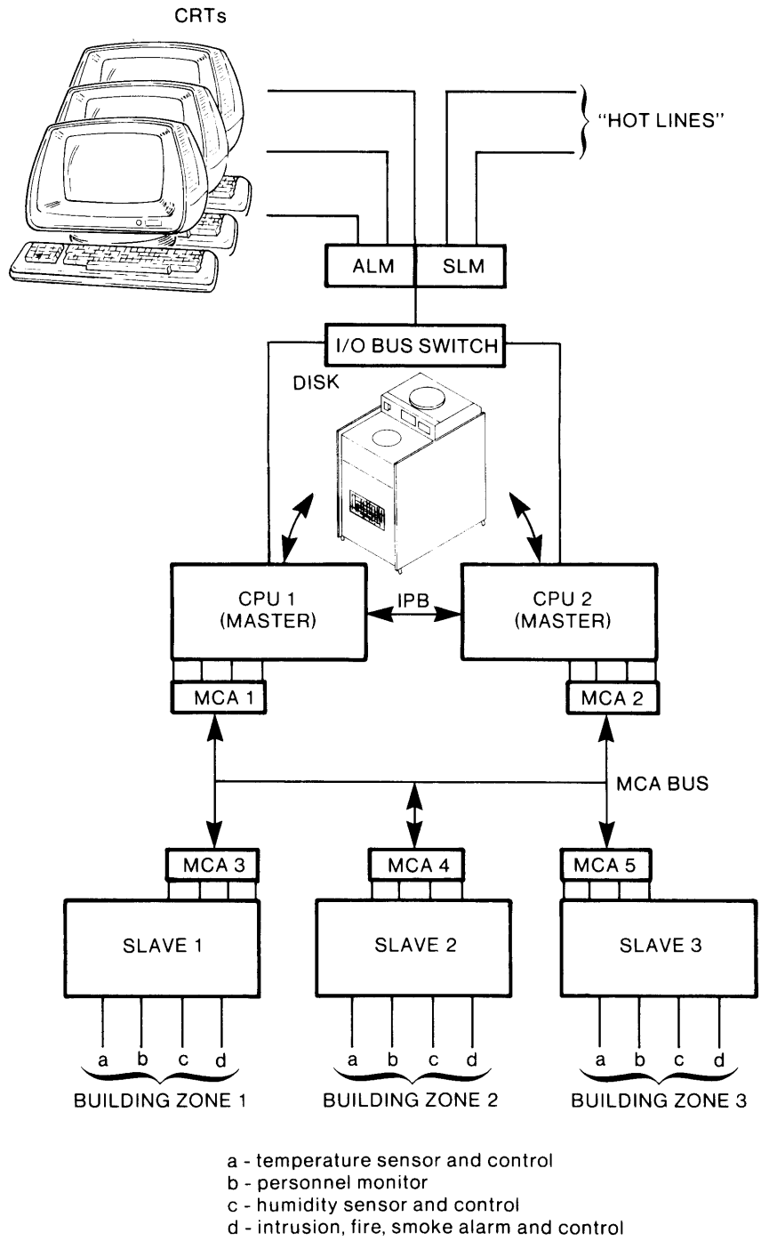
Figure 8.2 Multiprocessor system illustration
