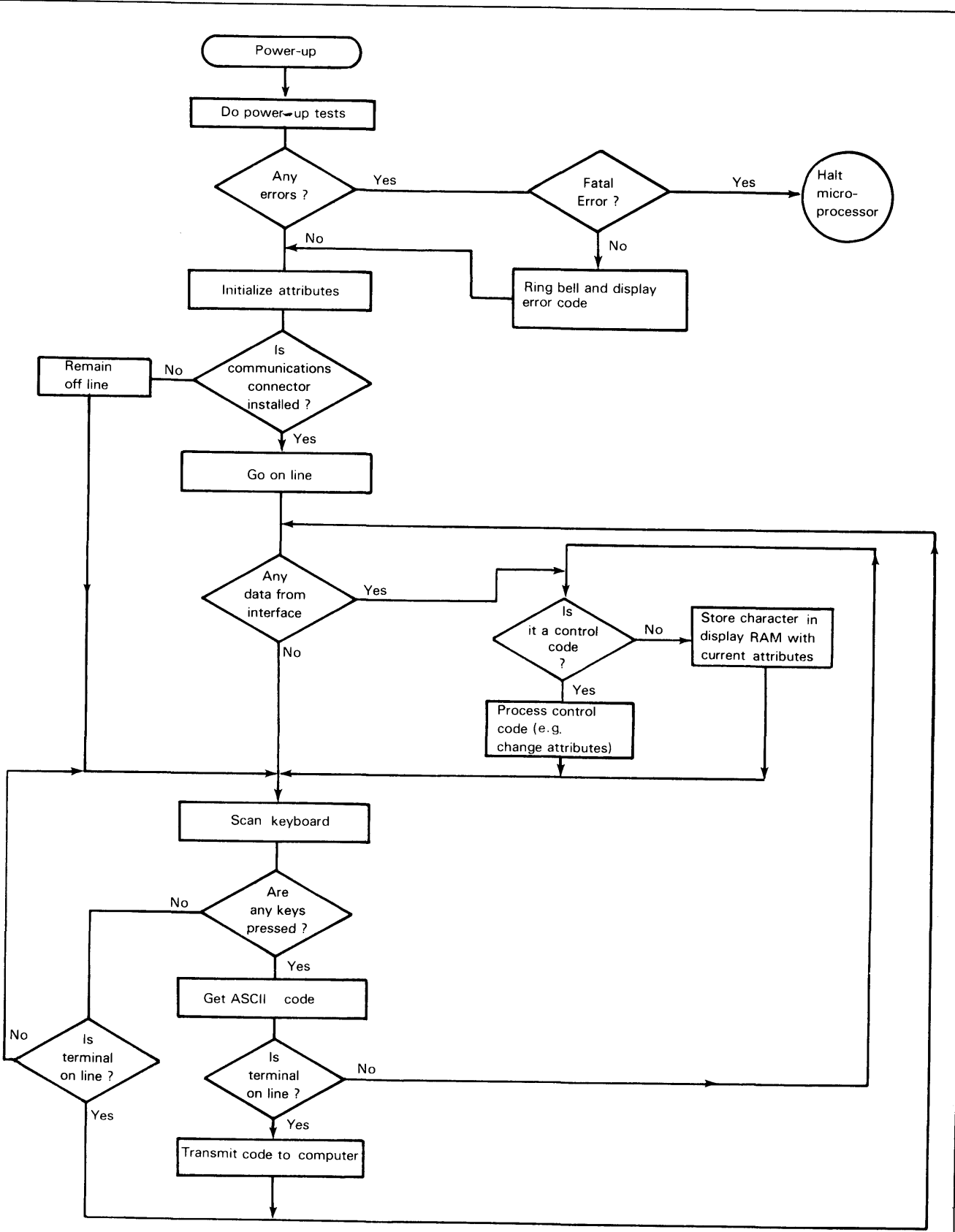
Figure 5.4 Functional Flow
