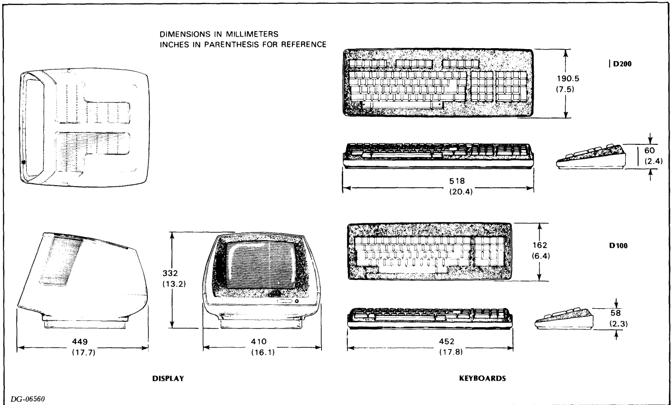
Figure 4.1 Terminal Dimensions
