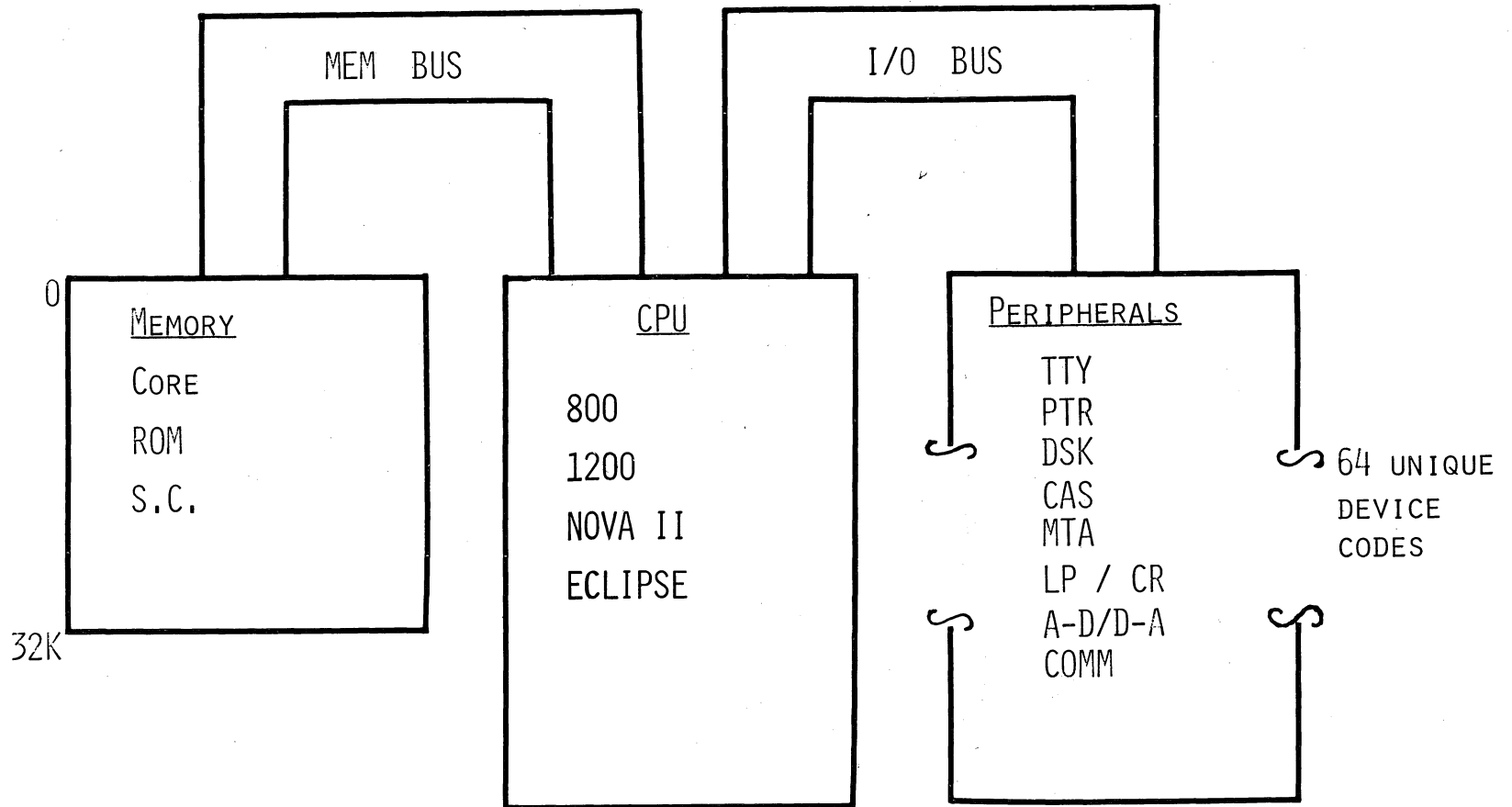
FIGURE 1-1. SYSTEM BLOCK DIAGRAM
