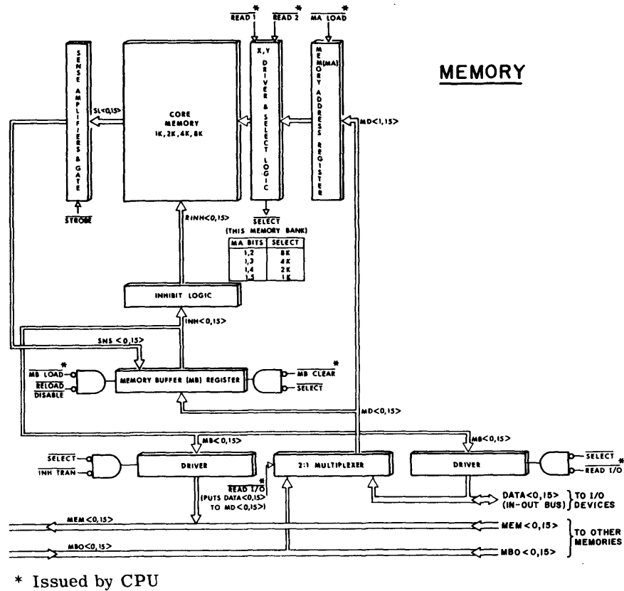
Figure M-3 Core Memory
