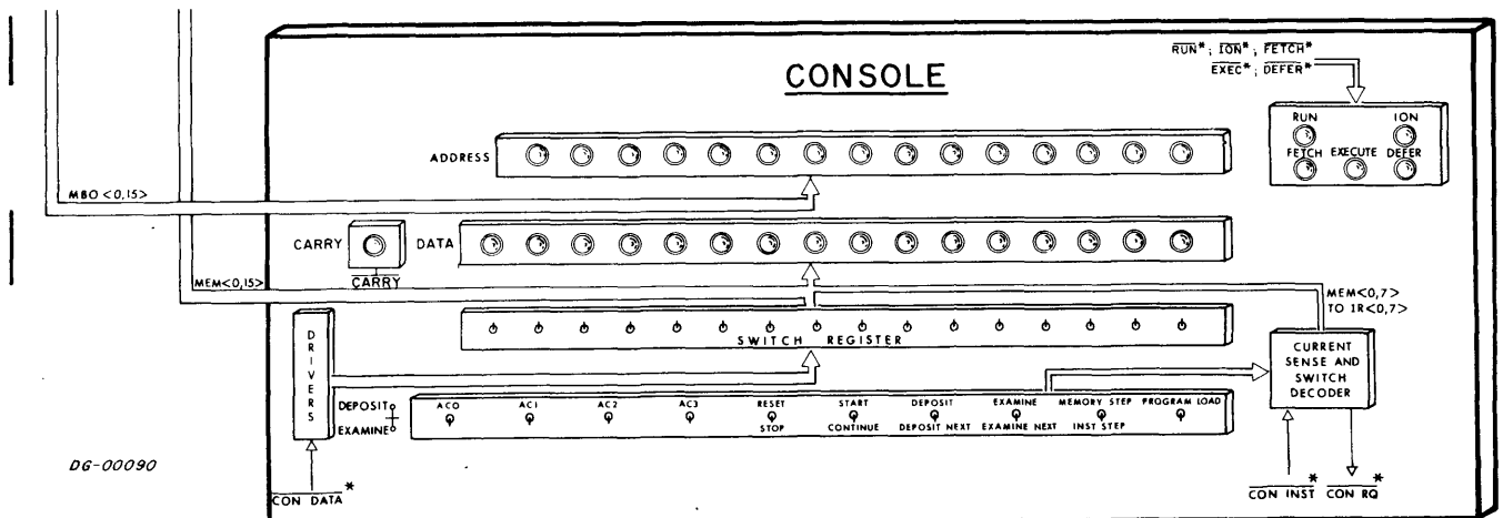
Figure K-1 The Console
